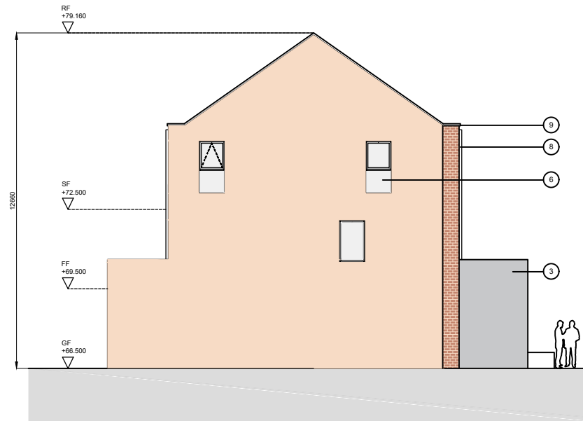
Side Elevation
