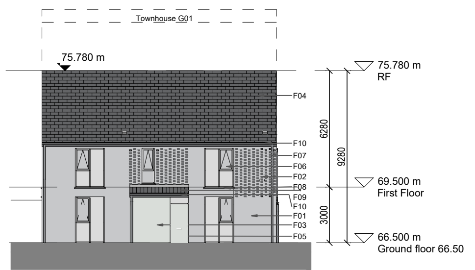
4 Side Elevation (North) - Block G - Townhouse 1 : 200
