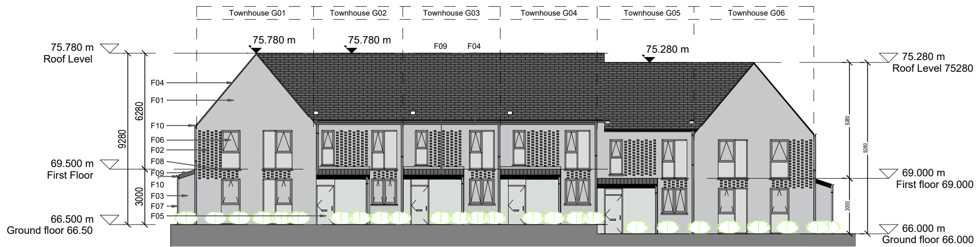
1 Front Elevation (West) - Block G - Townhouse 1 : 200
