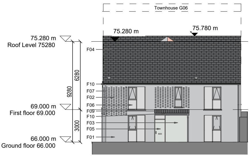
3 Side Elevation (South) - Block B - Townhouse 1 : 200
